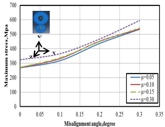
Figure (6) Effect of misalignment angle about z-axis
