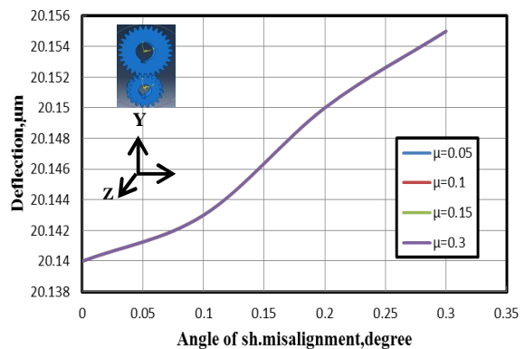
Figure (7) Effect of misalignment angle about z-axis
