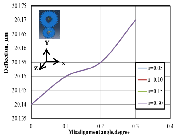
Figure (5) Effect of misalignment angle about Y-axis
