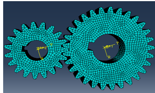
Figure 2 Mesh of spur gears
