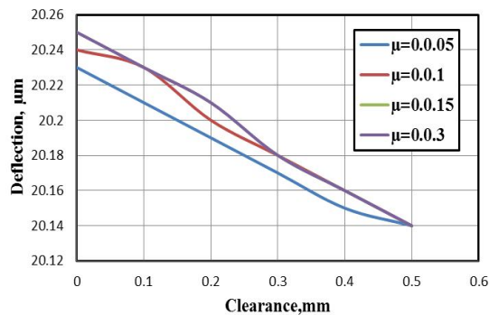
Figure (9) Effect of clearance at \mu=0.3 .
