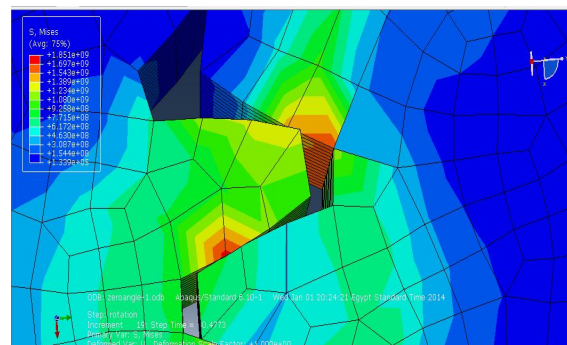
Figure 3 Maximum stress concentration
