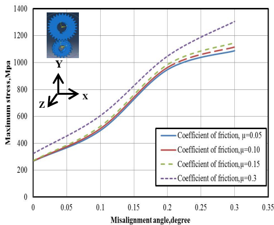
Figure (4) Effect of misalignment angle about Y-axis
