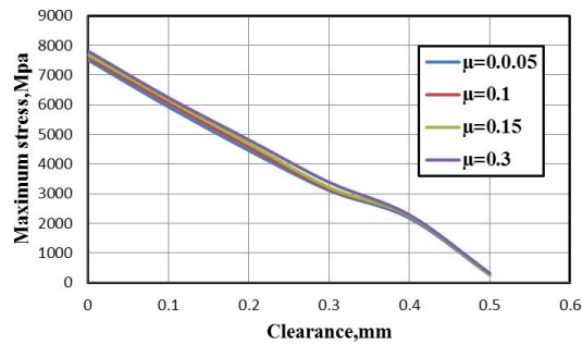
Figure (8) Effect of clearance at \mu=0.3 .
