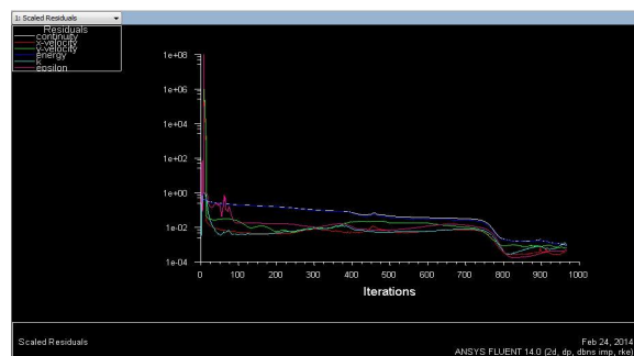
Fig. 3 Scaled Residuals
